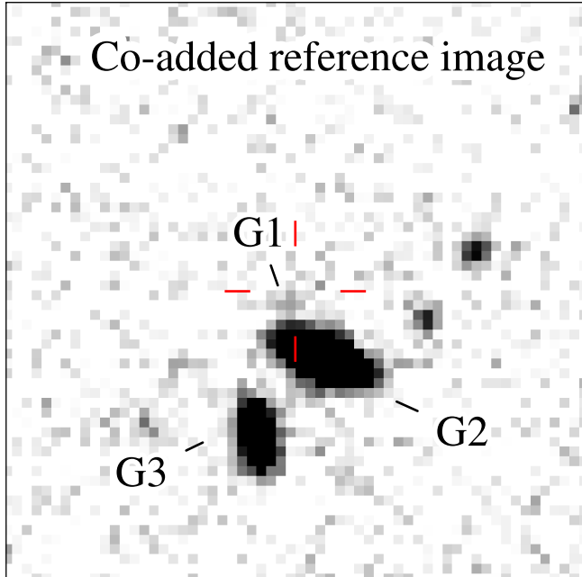
PTF field 3486, chip 1:1
