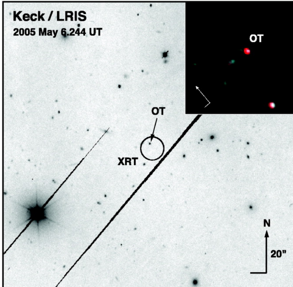
Fig. 1. from Spectroscopy of GRB 050505 at z = 4.275 : A \log N(\text{H I}) = 22.1 DLA Host Galaxy and the Nature of the Progenitor Berger et al. 2006 ApJ 642 979 doi:10.1086/501162 https://dx.doi.org/10.1086/501162 © 2006. The American Astronomical Society. All rights reserved. Printed in U.S.A.
