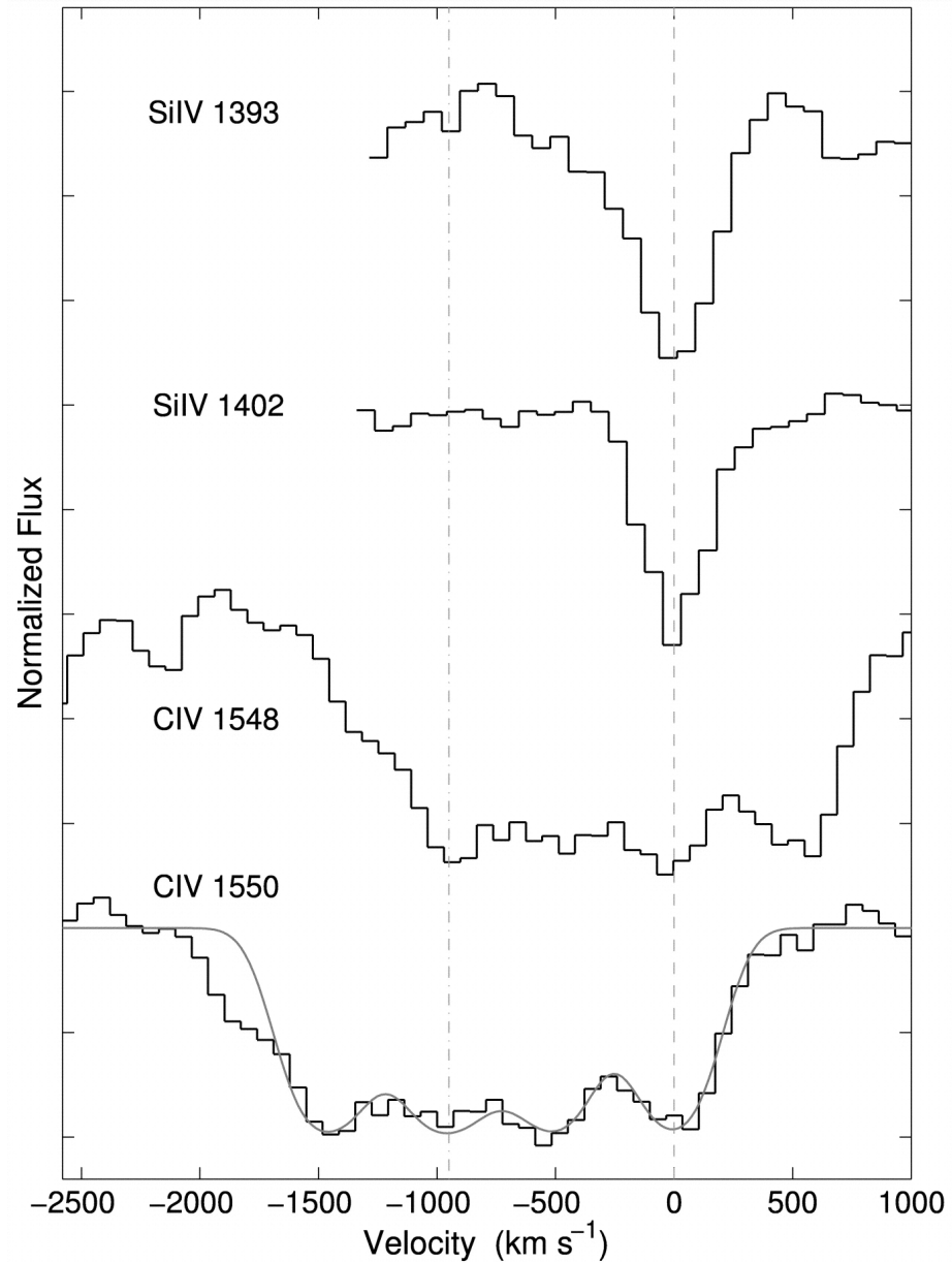
Fig. 5. from Spectroscopy of GRB 050505 at z = 4.275 : A \log N(\text{H I}) = 22.1 DLA Host Galaxy and the Nature of the Progenitor Berger et al. 2006 ApJ 642 979 doi:10.1086/501162 https://dx.doi.org/10.1086/501162
