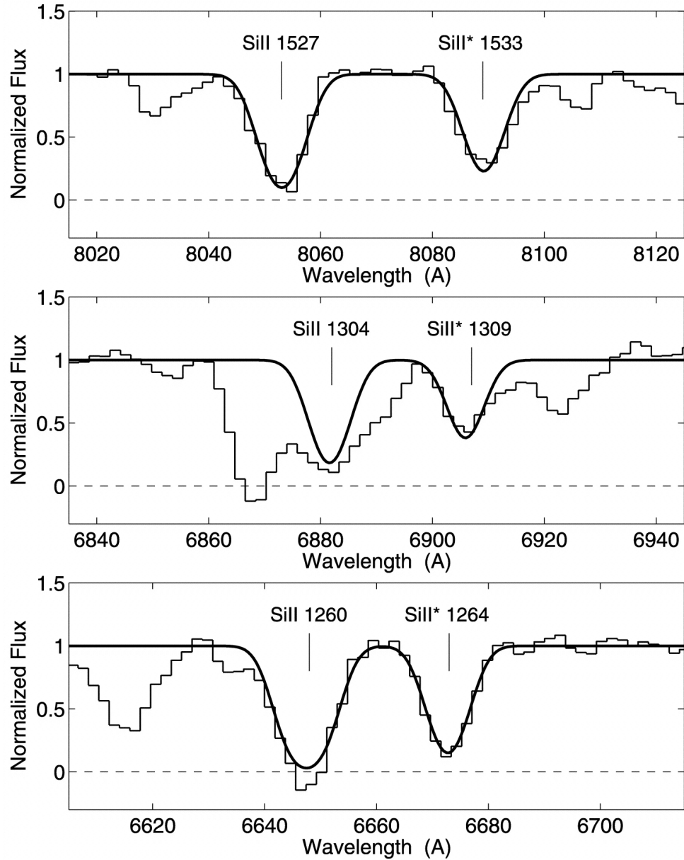
Fig. 6. from Spectroscopy of GRB 050505 at z = 4.275 : A \log N(\text{H I}) = 22.1 DLA Host Galaxy and the Nature of the Progenitor Berger et al. 2006 ApJ 642 979 doi:10.1086/501162 https://dx.doi.org/10.1086/501162 © 2006. The American Astronomical Society. All rights reserved. Printed in U.S.A.
